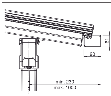
GP5200 | GP5210 Cross-beam set back, water channel mounted
