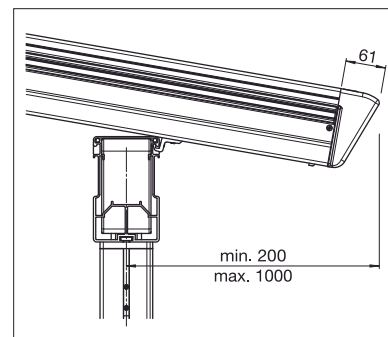
GP5300 | GP5310 Cross-beam set back without water channel
