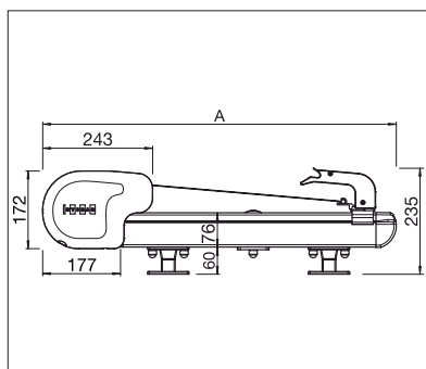
PS6000 Vista lateral
