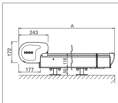
PS6100 Vista lateral
